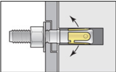
As bolt is tightened, it spreads to grip the sides of the hole.
