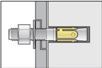
Insert bolt, place wall strap.
